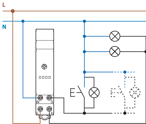
3 wire connection
