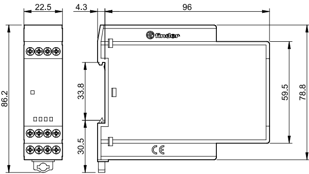
Type 75.63 Box clamp
