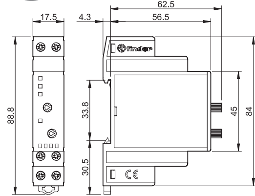
Type 19.3K/19.6K Screw terminal KNX terminal
