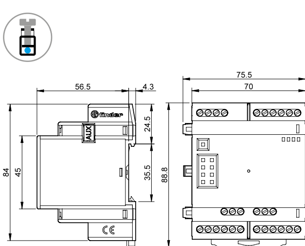
Type 8A.26-0600 Box clamp
