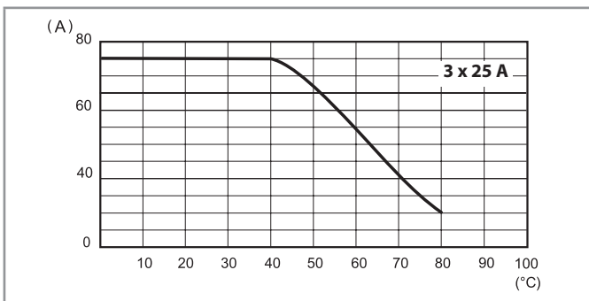
L77-22 Output RMS current v ambient temperature 77.A3.x.xxx.8671
