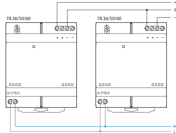
Series connection
