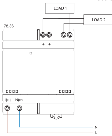
Basic connections
