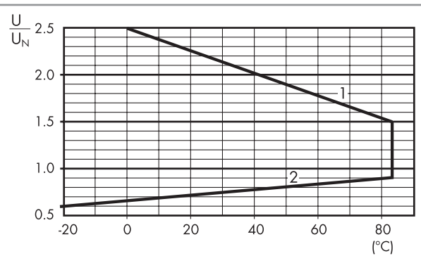
R 41 - DC coil operating range v ambient temperature
