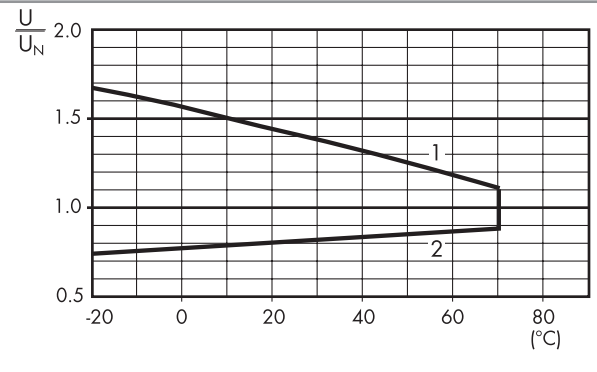
R 41 - AC coil operating range v ambient temperature
