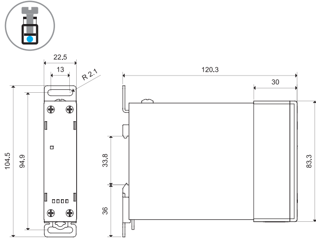
Types 77.11/21/31 Screw terminal
