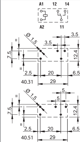
Copper side view Pin length 3.5 mm for PCB only Pin length 5.3 mm for PCB or sockets
