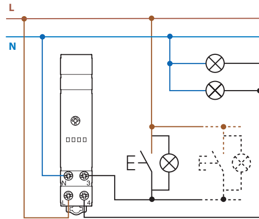
4 wire connection
