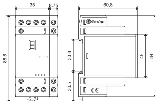
Types 22.34 + 022.33/022.35 Screw terminal
